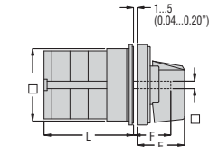
Front ring mount on Ø22mm drilling, 2-screw fixing
