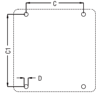
Drilling for enclosure fixing
